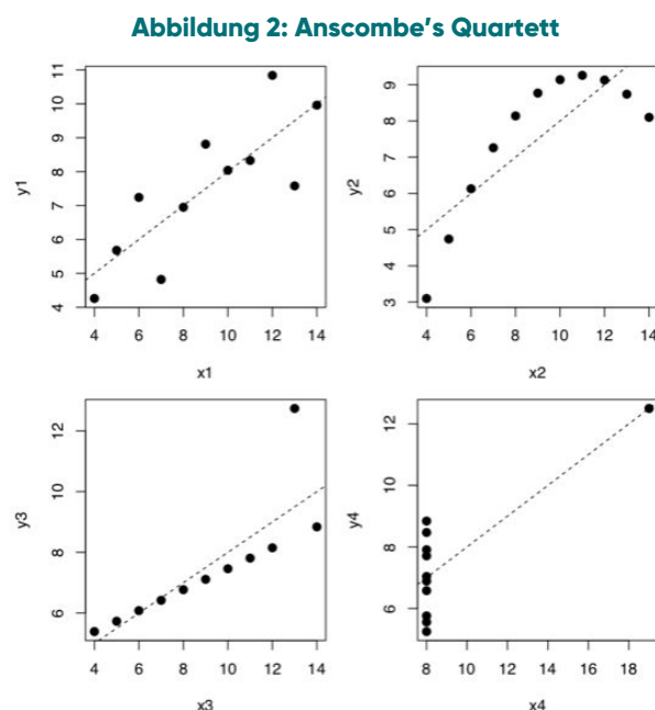
Figure 6.1.2 Anscombe's quartet, plotted together with lines from linear models.
